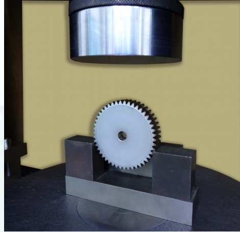
Universal Strength Tester
