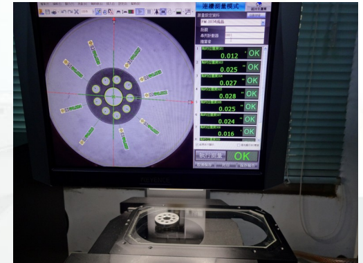
Automatic Profile Projector
